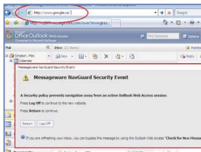
Navigation detected when the users enters a new URL in the address bar
